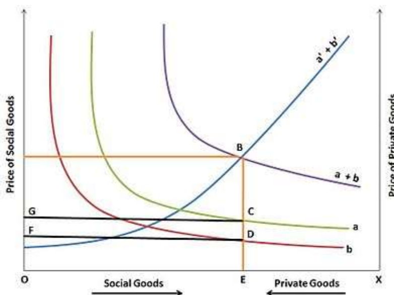
Figure 4: Bowen's Model
